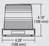
PERMANENT MOUNT
